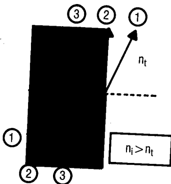
Figure 0.7. Geometry of total internal reflection. Ray #1 is at less than the critical angle. Ray #2 is at the critical angle. Ray #3 is totally internally reflected.
