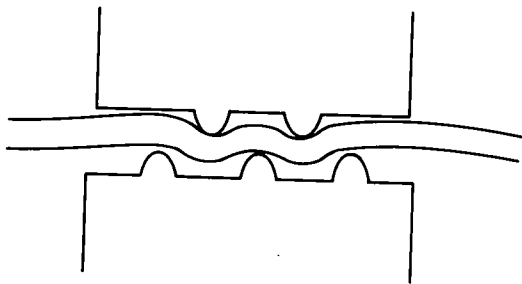
Figure 0.17. Mode scrambler for optical fibers. The bends tend to couple out higher-order and radiation modes and to distribute the light into a distribution of modes that will remain stable over long distances.
