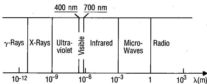
Figure 0.4. The electromagnetic energy spectrum.
