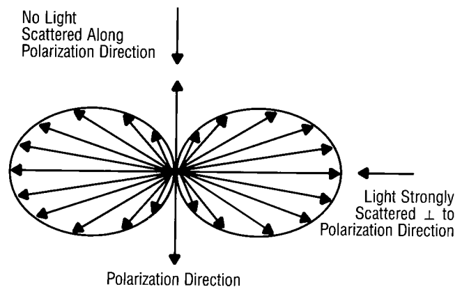
Figure 0.20. Scattering of light by a linearly-polarized field (dipole). Light is scattered strongly at right angles to the dipole direction, but is not scattered at all along the direction of the electric field vector.
