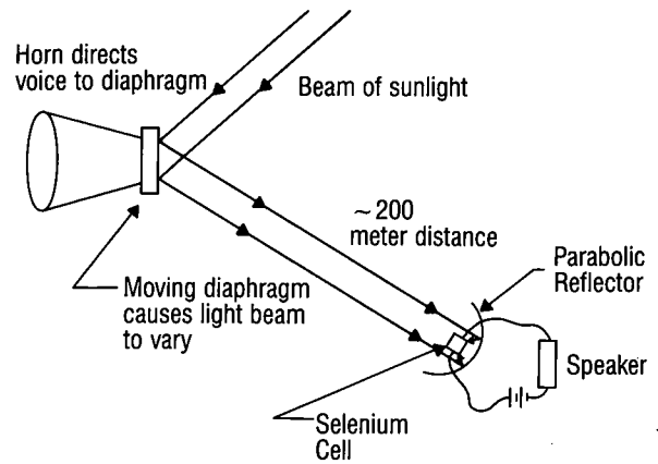
Figure 0.1. Schematic diagram of Alexander Graham Bell's photophone.
